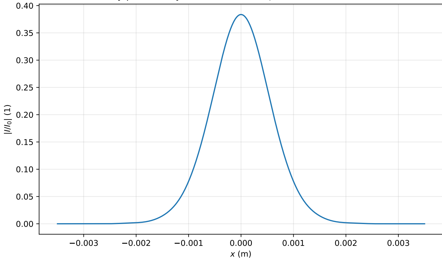
Intensity profile I(x, y = 0, z = 3.582m)/I_0 , P_{in}=0.4P_{cr} , artificial time
